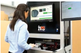
Object: Optical Inspection of PCB board Machine reads the component's datamatrix serial number and checks the part's body for surface defects.
