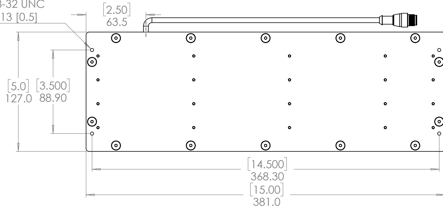
BOTTOM VIEW
